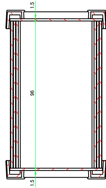
C-C (1:1.5)
