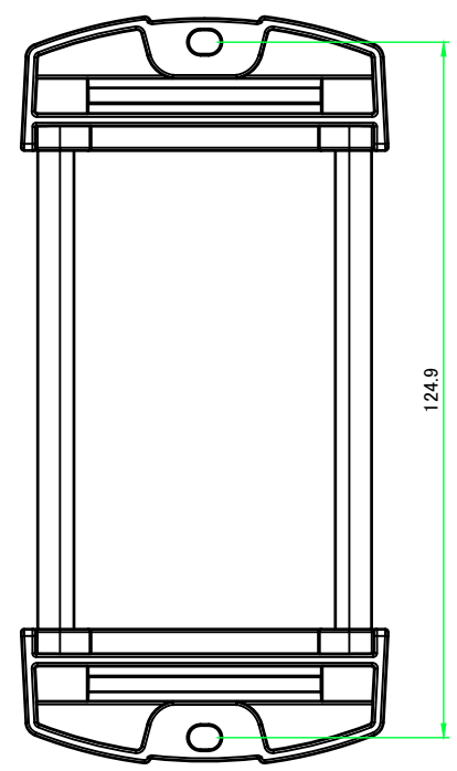
C-C (1:1.5)
